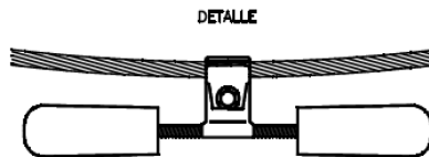
Figura 14: Antivibrador Stockbridge.
