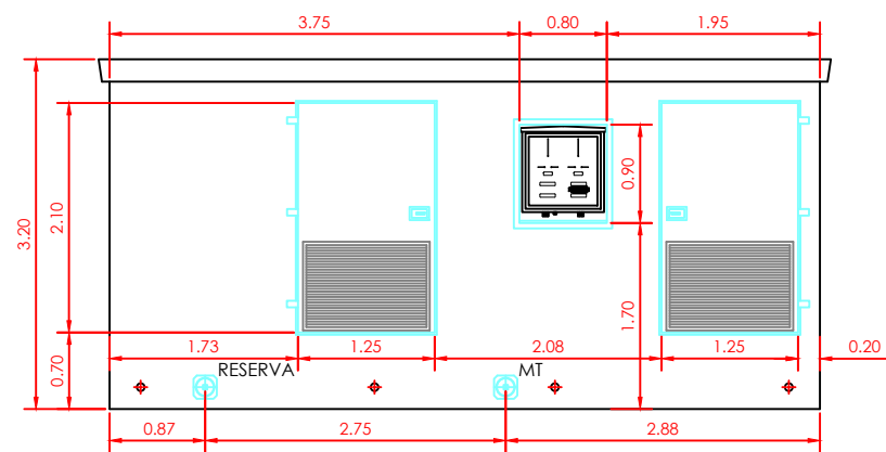
ALZADO PRINCIPAL
