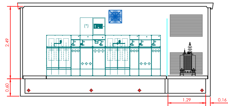
ALZADO PRINCIPAL
