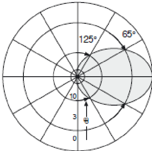
Horizontal Pattern
