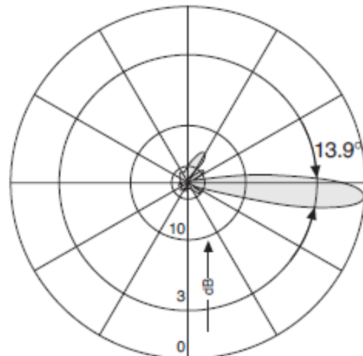
Vertical Pattern
