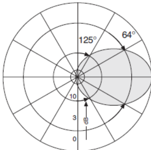
Horizontal Pattern
