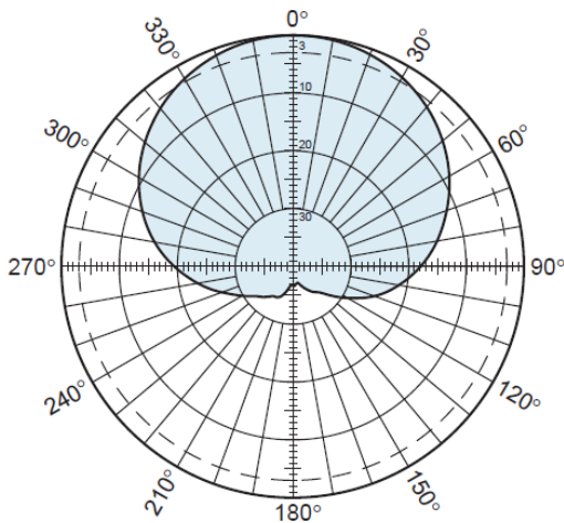
Horizontal pattern \pm 45^\circ - polarization
