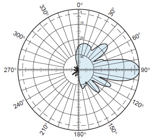
Vertical pattern \pm 45^\circ - polarization 0^\circ - 14^\circ electrical downtilt
